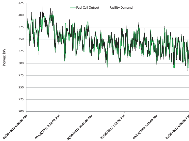
Figure 3. Load-Following Operating Data for Net Metering Site
